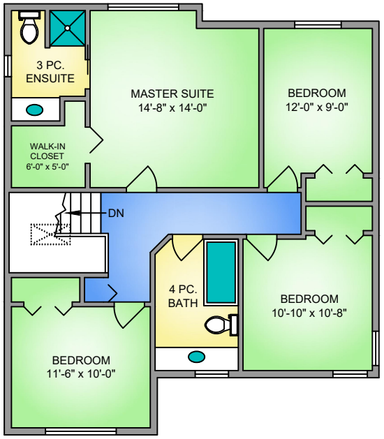
UPPER FLOOR 994 SQ. FT. 8' CEILING HEIGHT
