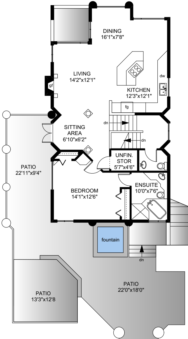
MAIN FLOOR 1081 SQ.FT
