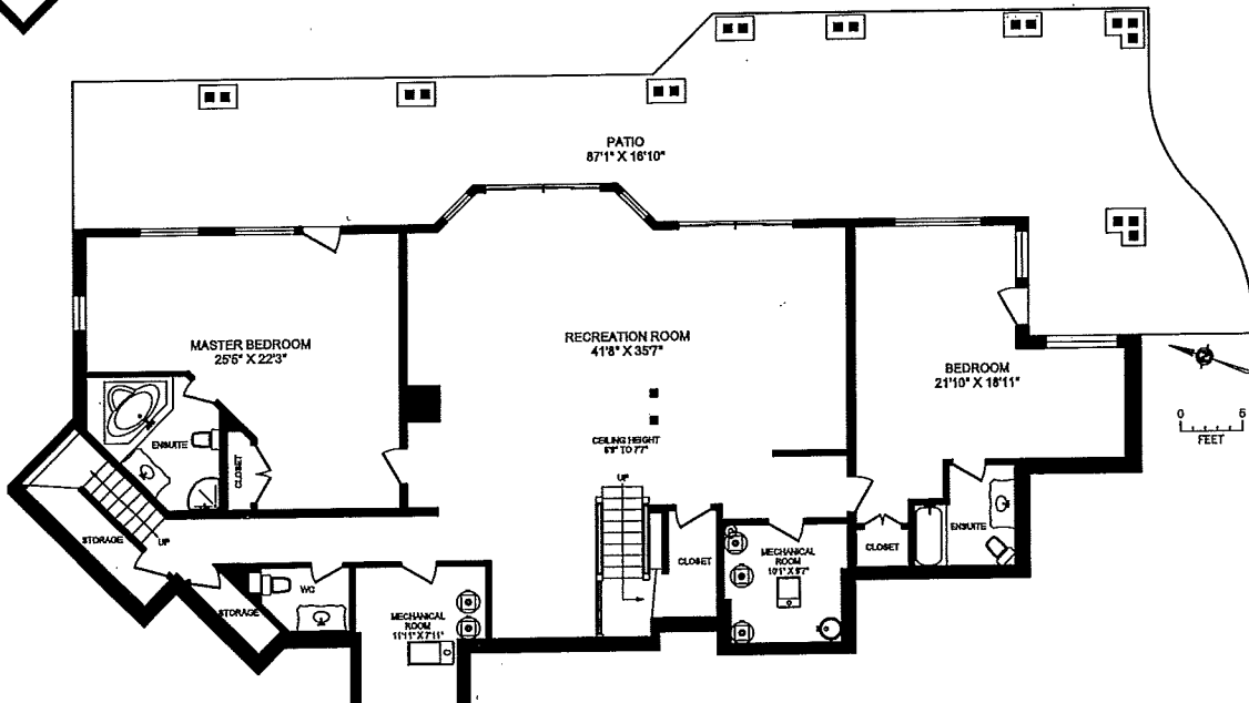
LOWER FLOOR
